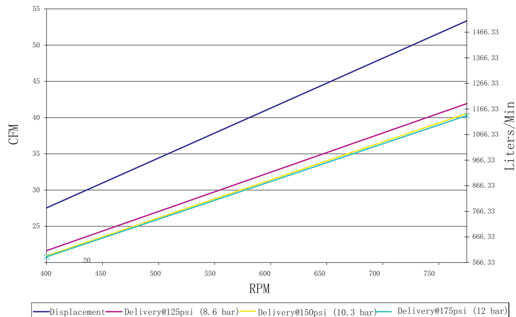
LP352 Performance (Delivery)
