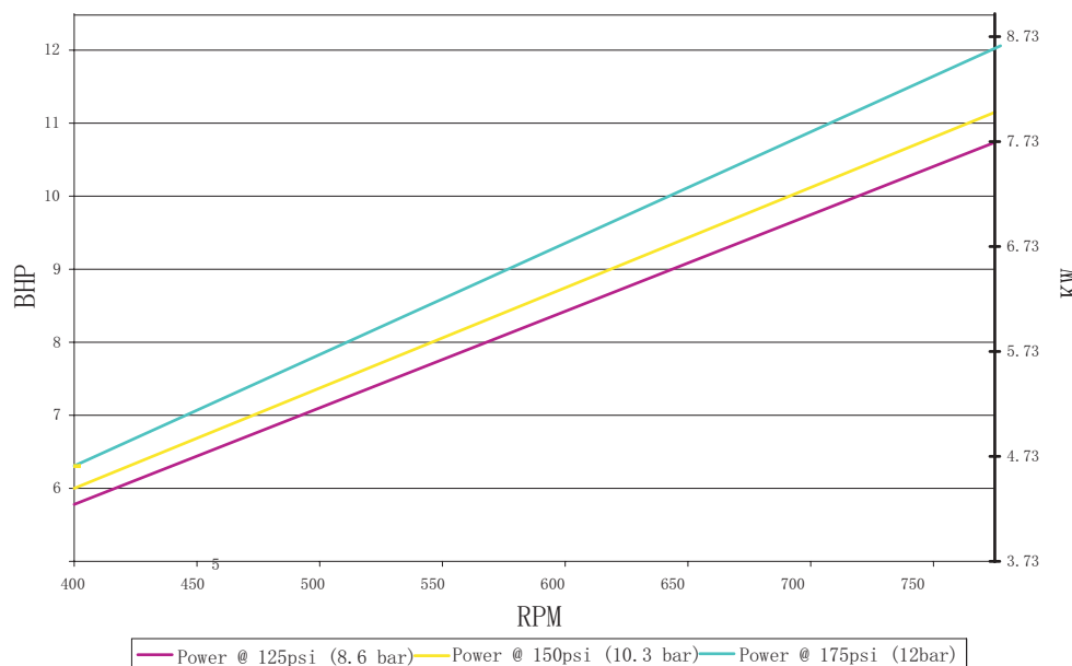
LP352 Performance (Power)
